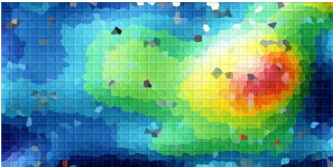
Granulated (domain/group) broken up mud field
