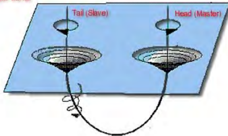
Schematic view of a Falaco soliton
