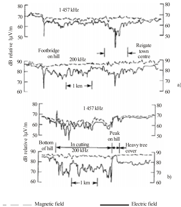
Measurements on two routes with magnetic and electric antennas
