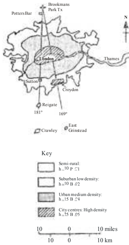
FIGURE 17 Measurement paths across London
