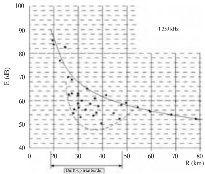
FIGURE 33 Field strength variability in built up areas at 1 359 kHz
