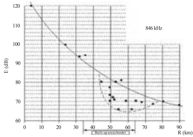
FIGURE 32 Field strength variability in built up areas at 846 kHz
