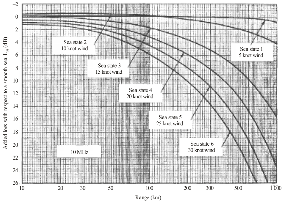
FIGURE 8 Sea state losses at 10 MHz
