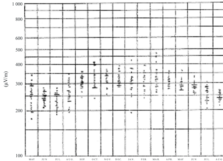
FIGURE 20 Example of seasonal variation recorded in USA
