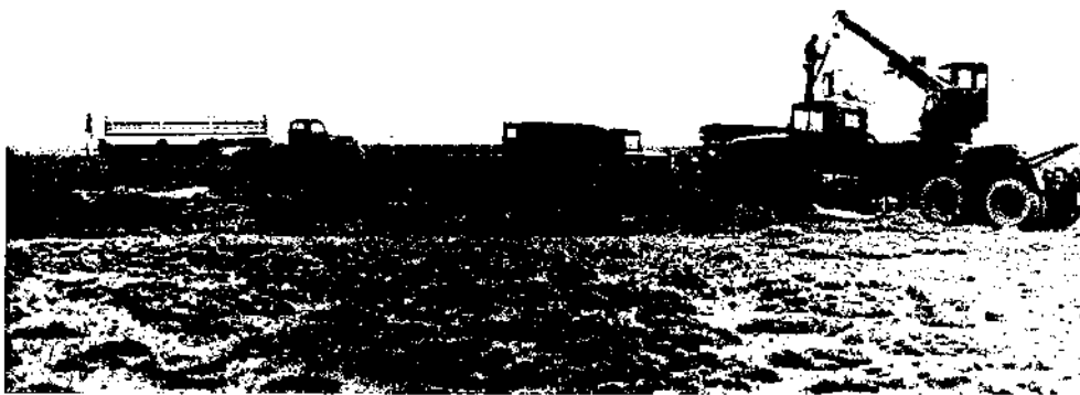
Fig. 80. Witnesses described a “tanker,” “military ambulances,” a “6x6,” and a “wrecker”—probable references to (from left) a helium tank trailer, a M-43 ambulance (converted to a communications vehicle), a M-35 cargo truck (partially obscured), and a M-342 wrecker. These vehicles were used for off-range launch and recovery operations of anthropomorphic dummies for Project HIGH DIVE/EXCELSIOR. Shown here is a May 29, 1957 dummy launch near Hatch, N.M. (also see figs. 23, 28, 64, 71, 81). (U.S. Air Force photo)
